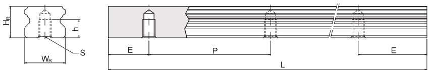
(5) Dimensions for ER-T (rail mounting from bottom)
